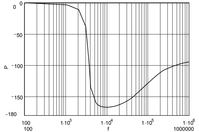
Figure 6. The Phase Curve with ESR = 0.002Ω
